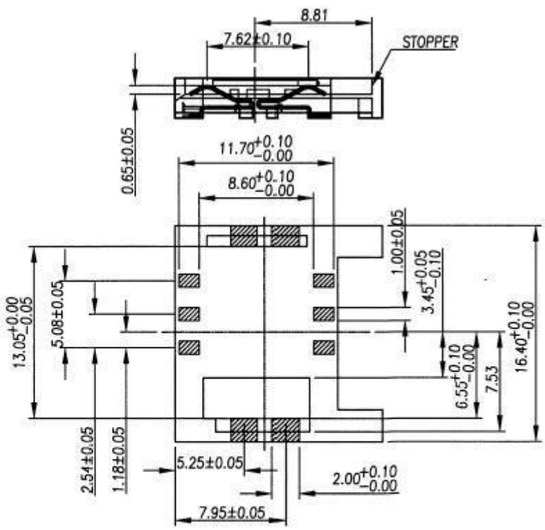
P.C.B. LAYOUT (TOLERANCES: \pm 0.10 mm)
