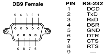
RS-232 Pin Assignment Diagram
