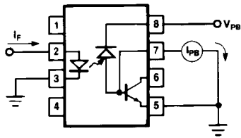
Figure 2. Base Photo Current Test Circuit.
