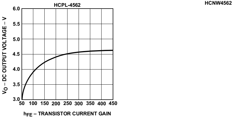
Figure 15. DC Output Voltage vs. Transistor Current Gain.
