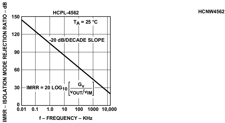
Figure 14. Isolation Mode Rejection Ratio vs. Frequency.
