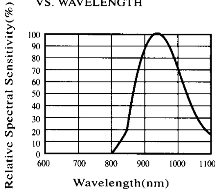
Fig-1 RELATIVE SPECTRAL SENSITIVITY VS. WAVELENGTH
