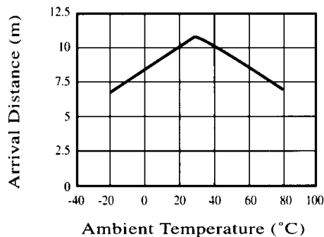
Fig-6 ARRIVAL DISTANCE VS. AMBIENT TEMPERATURE
