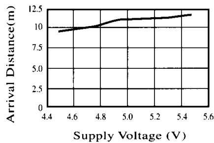
Fig-4 ARRIVAL DISTANCE VS. SUPPLY VOLTAGE
