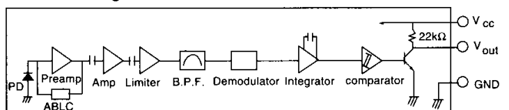
Block Diagram:
