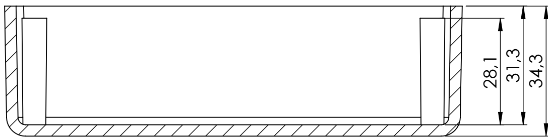
SECTION B-B
